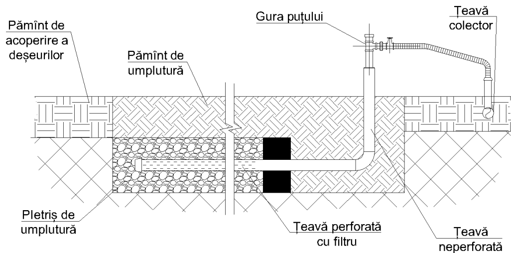
Figura 5 - Colector de gaze orizontal
